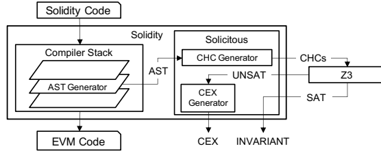
Fig. 4. Solicitous module inside the Solc compiler.
