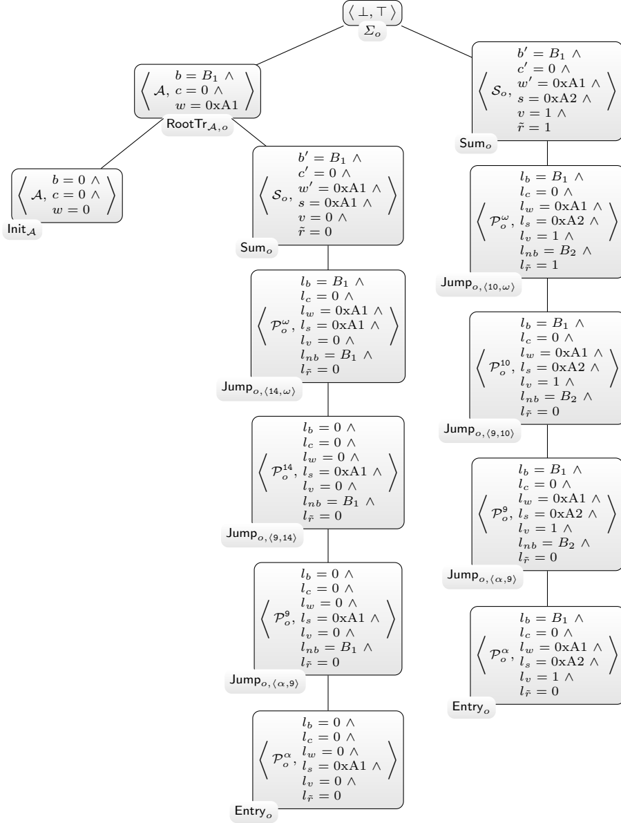
Fig. 3. A refutation tree for the set of CHCs shown in Fig. 2 modelling the contract Auction shown in Fig. 1. \Sigma_o is the CHC \mathcal{A} \wedge \mathcal{S}_o \wedge \tilde{r} \implies \perp . B_1 = 2^{256} - 5 \times 10^{15} , and B_2 = 2^{256} - 5 \times 10^{15} + 1 . The values 0xA1 and 0xA2 represent two Ethereum addresses.
