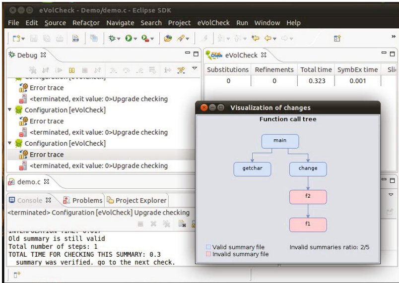
Fig. 7. eVolCheck change impact
